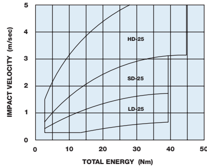
25mm Bore
