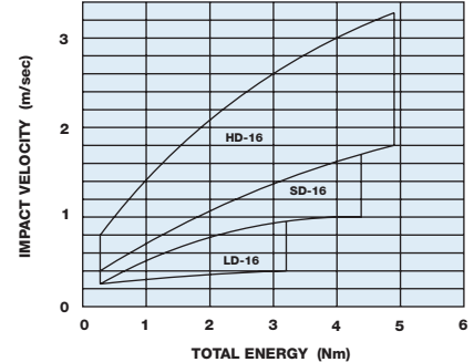
32mm Bore
