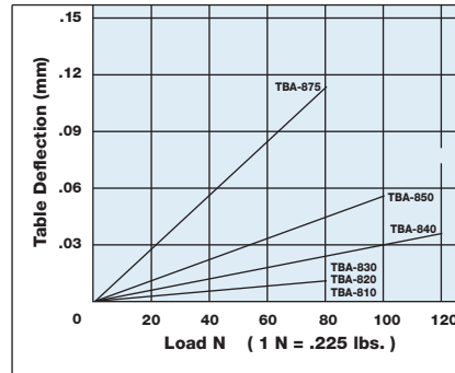
TBA-8
