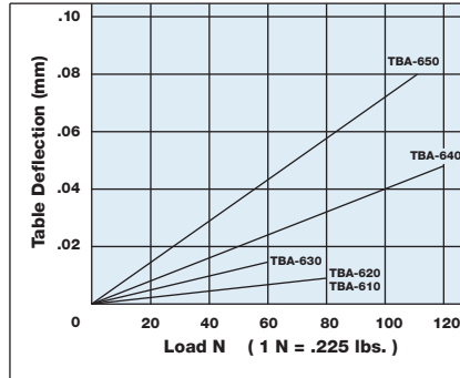
TBA-6
