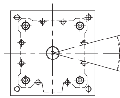
Non-Rotational Accuracy
