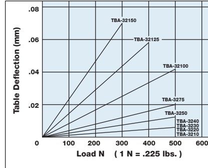
TBA-32
