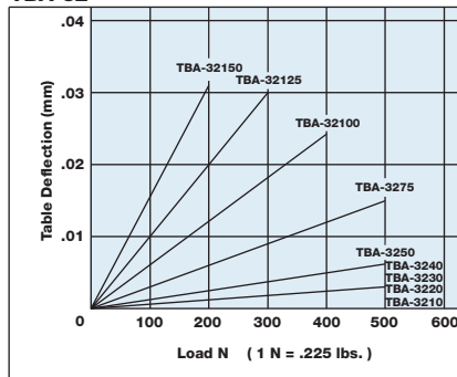
TBA-32
